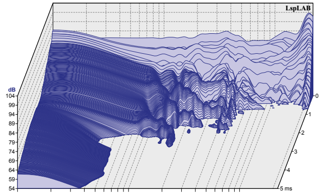
FR070WA02_SPL_frequency_response Description: Waterfall Acquire date: <Unknown>
