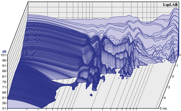
FR070WA01_SPL_frequency_response Description: Waterfall Acquire date: <Unknown>
