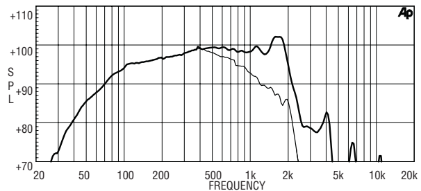
FREQUENCY RESPONSE CURVE OF 15LW1400 MADE ON 125 Lt. ENCLOSURE TUNED 50Hz IN FREE FIELD ( 4pi) ENVIRONMENT. ENCLOSURE CLOSE THE REAR OF THE DRIVER. THE THIN LINE REPRESENTS 45 DEG. OFF AXIS FREQUENCY RESPONSE
