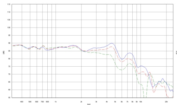
The frequency responses measured free field sound pressure in 0, 15 30 degrees angle using endless baffle. Input 2,83 VRMS, microphone distance 1 m
