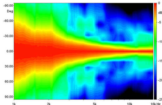
VERTICAL BEAMWIDTH
